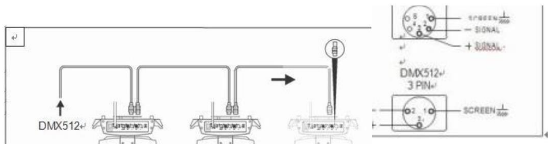
Figure 2 DMX signal connection
