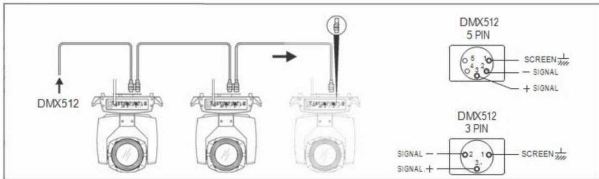
Figure 1 Diagram of the DMX Cable connection
