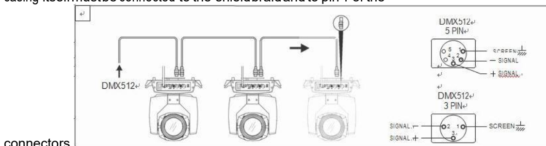
Figure 1 DMX Cable connection
